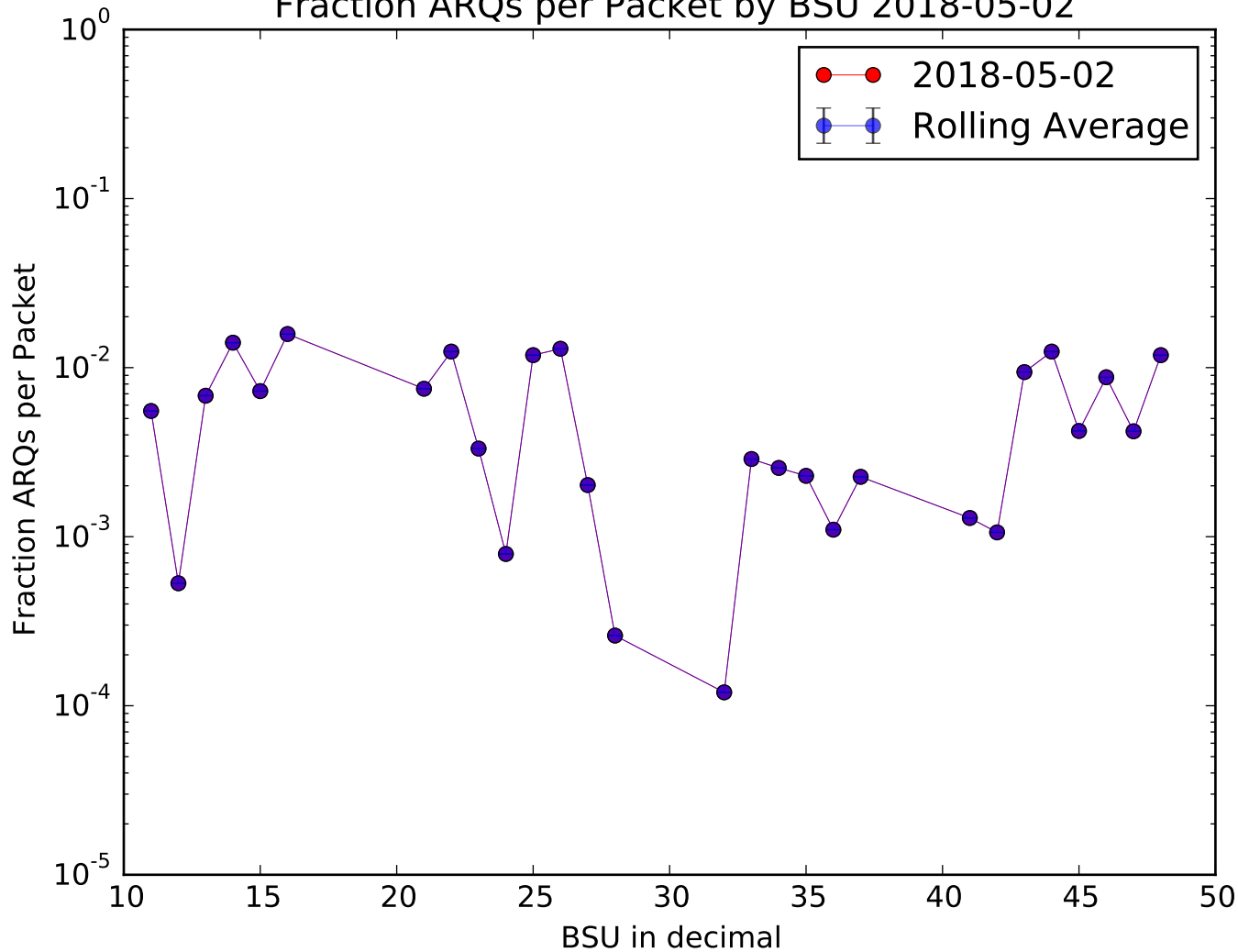
Fraction ARQs per Packet by BSU 2018-05-02
