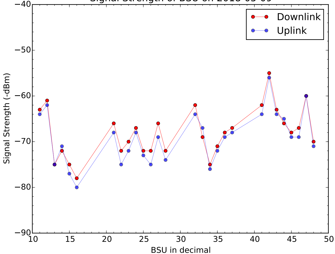
Signal Strength of BSU on 2018-05-09
