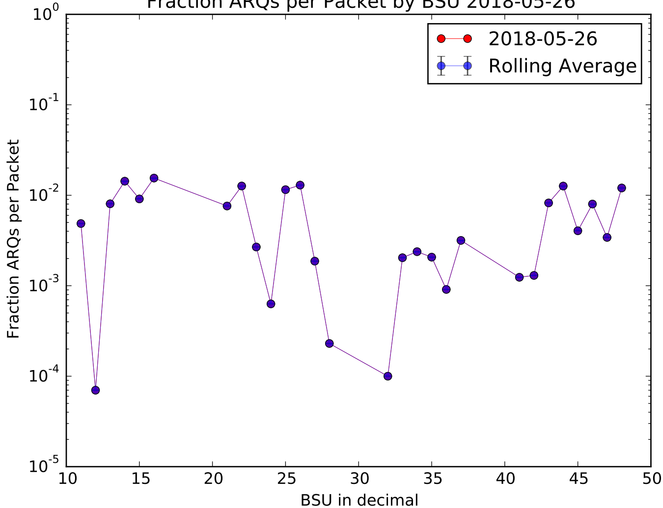
Fraction ARQs per Packet by BSU 2018-05-26
