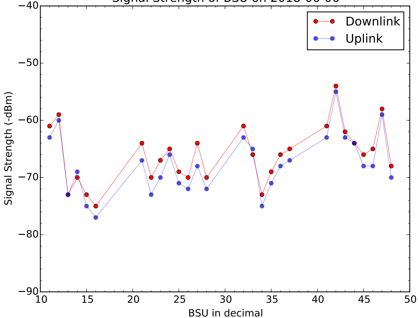
Signal Strength of BSU on 2018-06-06
