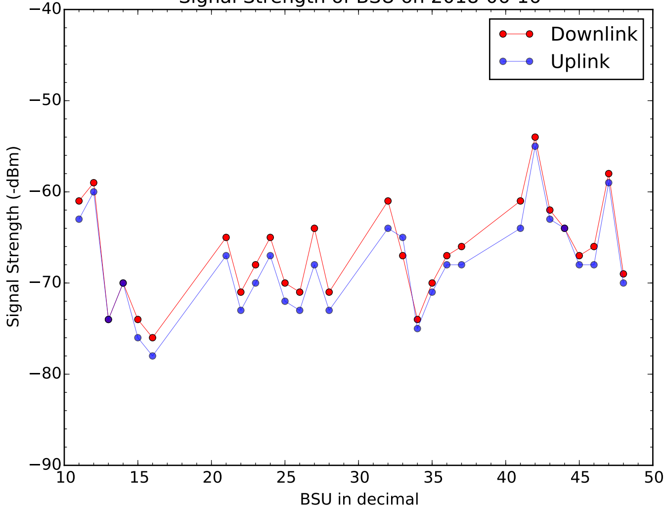
Signal Strength of BSU on 2018-06-16
