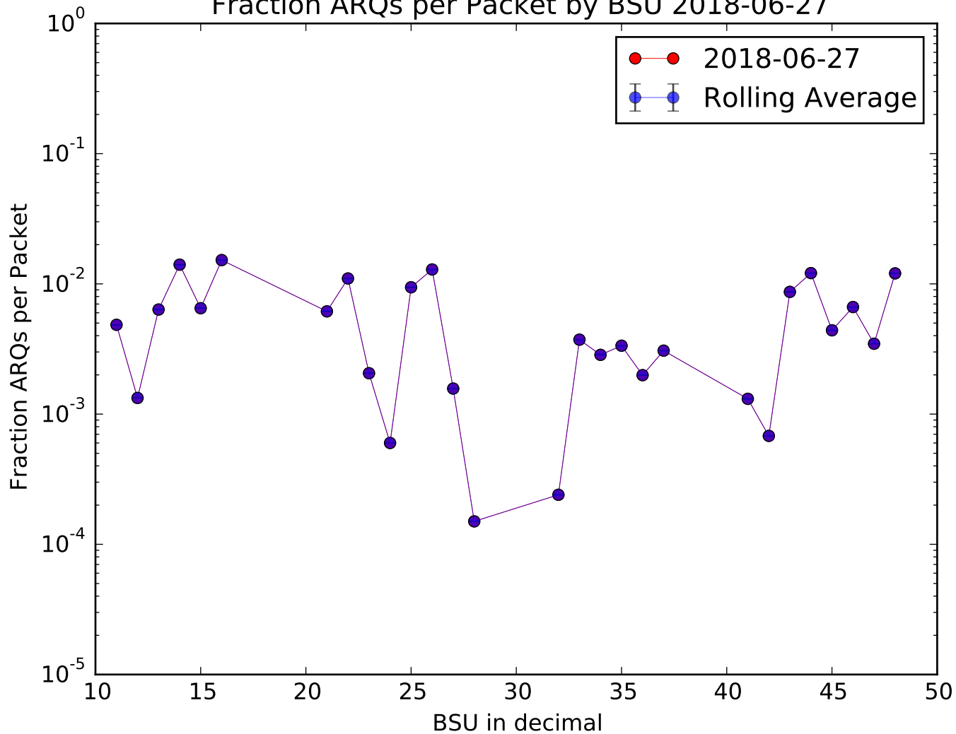
Fraction ARQs per Packet by BSU 2018-06-27
