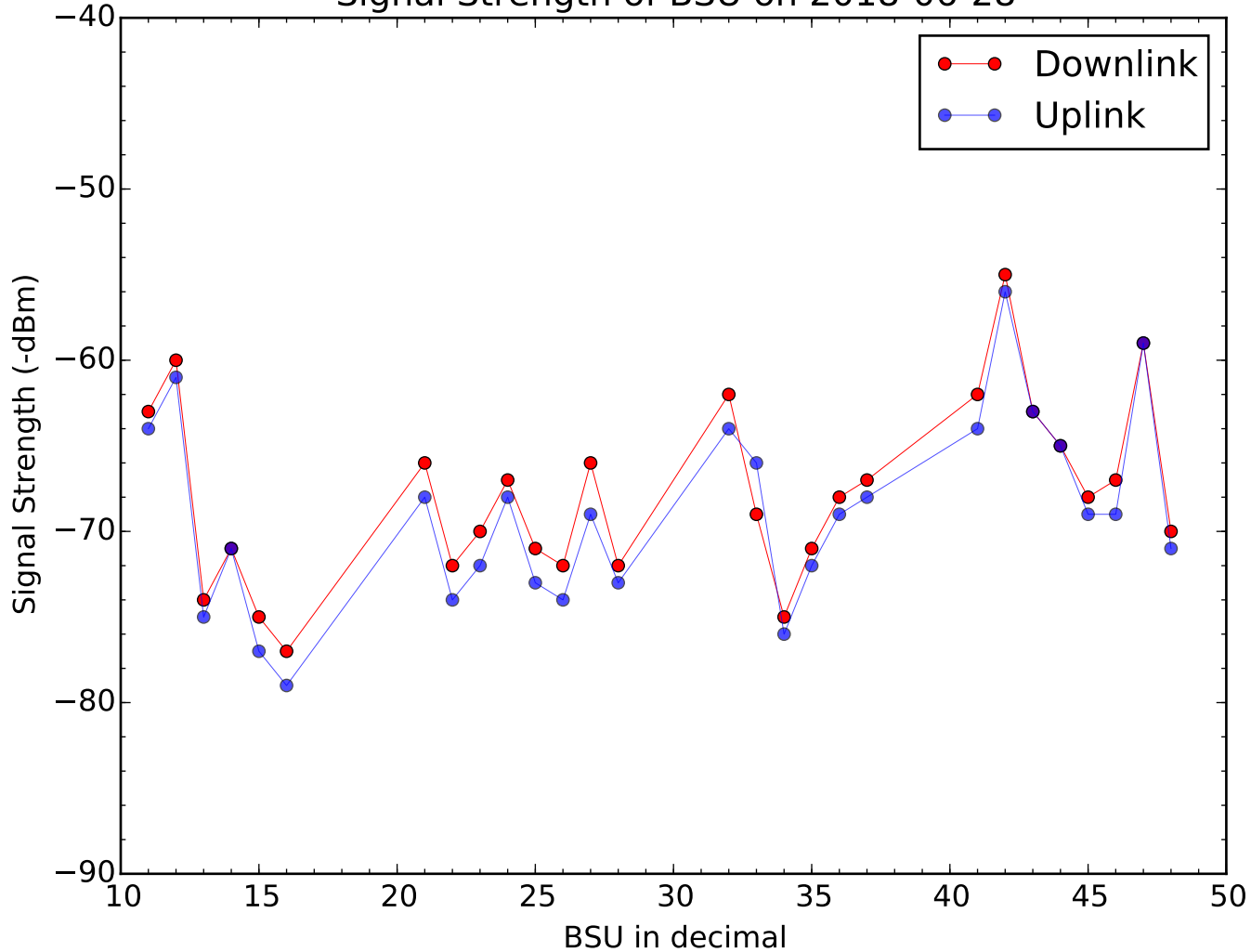
Signal Strength of BSU on 2018-06-28
