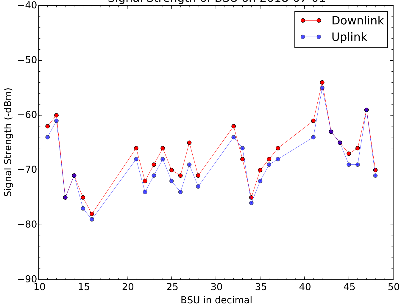
Signal Strength of BSU on 2018-07-01
