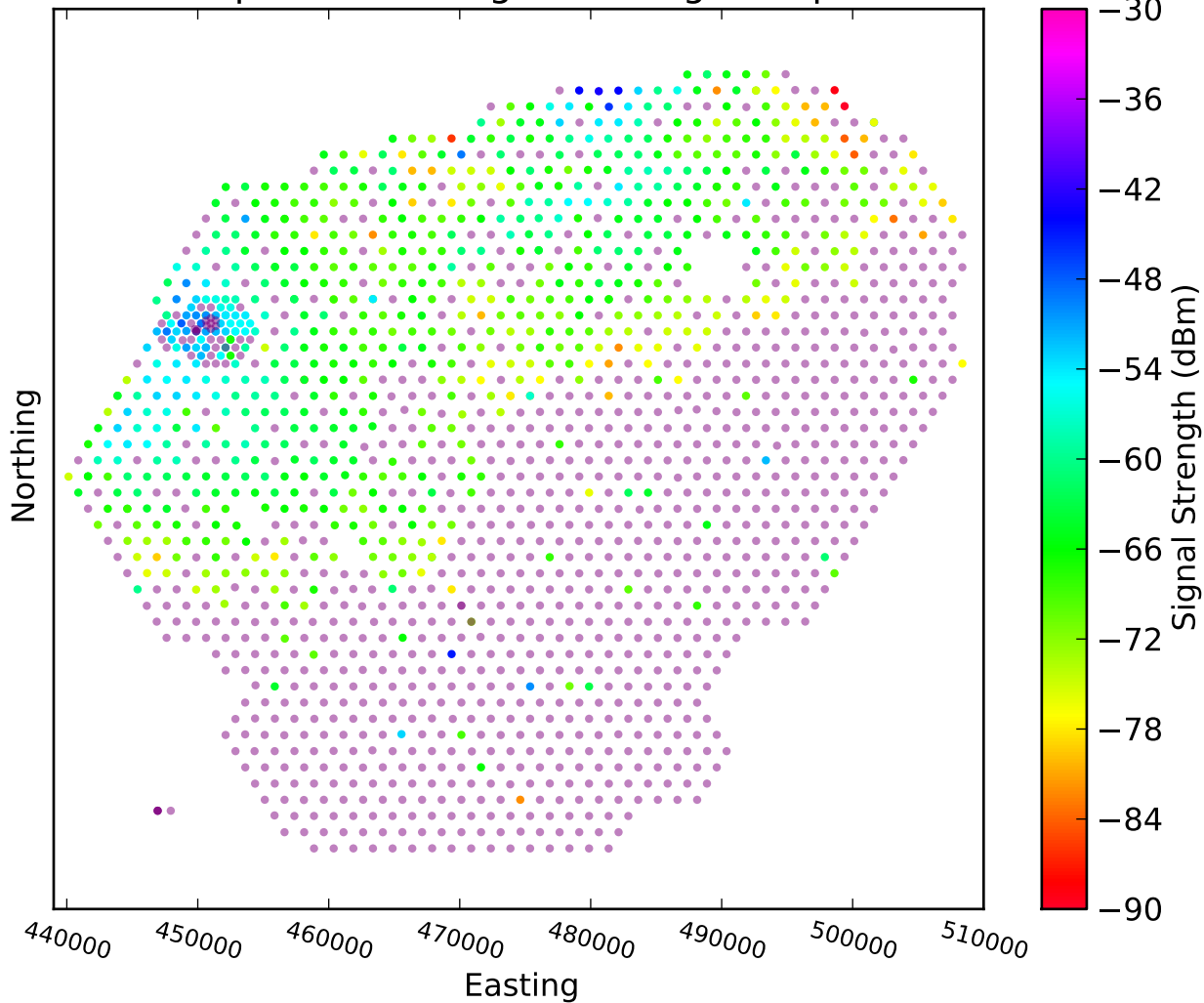
Uplink Radio Signal Strength Map
