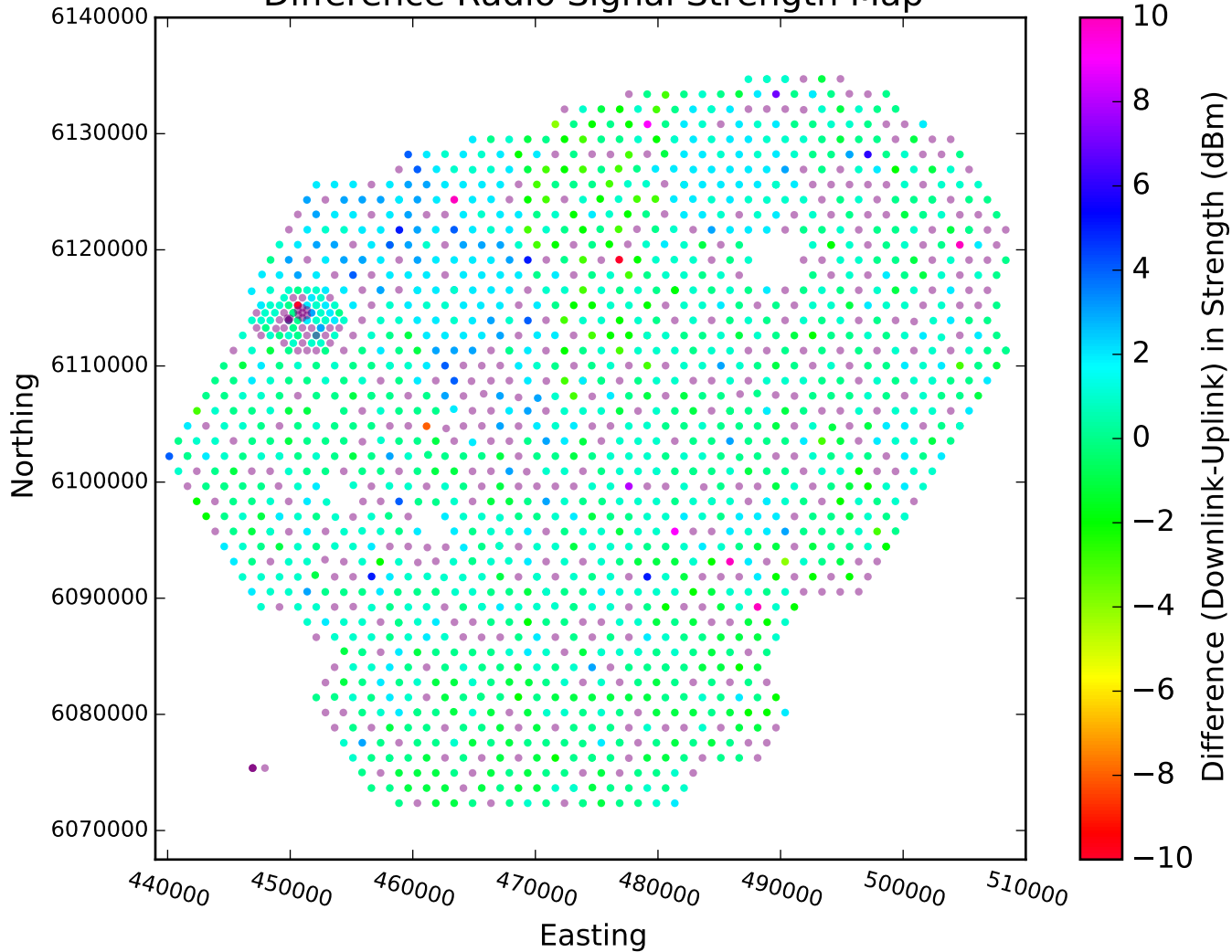
Difference Radio Signal Strength Map
